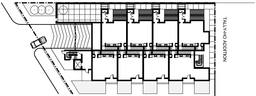
1 BLOCK A / UNIT PLAN / GROUND SCALE: 1/8" = 1'-0" DATE: JUNE 01, 2008
